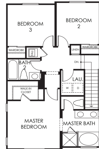
THIRD FLOOR
